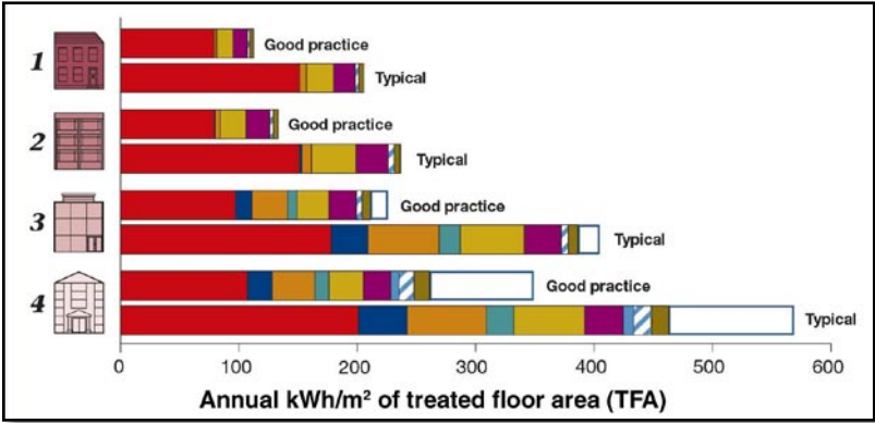
Energy use indices (EUIs) for good practice and typical examples of the four offices types
